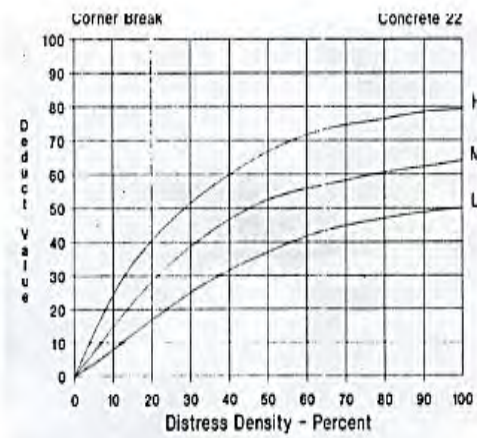
Figure 2-21 Corner break
